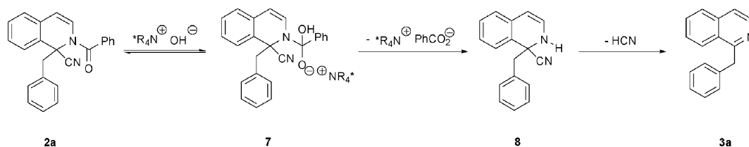
Scheme 3 Proposed reaction between 2a and *R 4 NOH.
